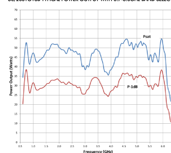
30/20S1G18B TYPICAL POWER OUTPUT WITH 0.7-6.0GHz BAND SELECTED
